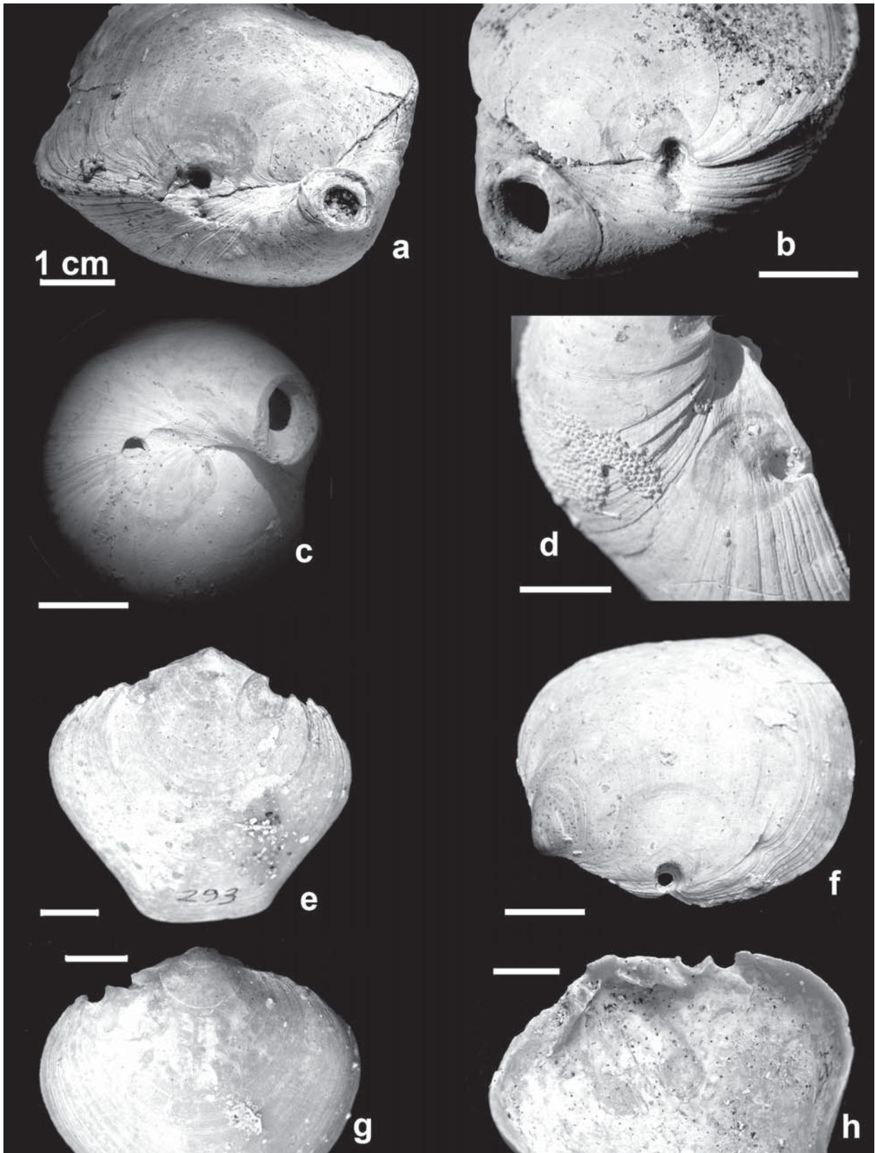
Figure 3. Oichnus taddeii isp. nov. All specimens are on Terebratula scillae shell from the Calabrian sands near Gallina (Reggio Calabria, Southern Italy). a) Holotype: trace n° 2063. b) Paratype 1, n° 343. c) Paratype 2, n° 323. d) Paratype 4, n° 345, the brachiopod reacted by growing shell tissue around the hole. e) Trace n° 293, the hole occurs in between the two valves. f) n° 502, a hole affecting a single valve. g-h) sp. 306, two holes and associated scars, partly overlapping; (g) outer, and (h) inner side of the dorsal valve of the brachiopod host. All scar bars are 1 cm.
